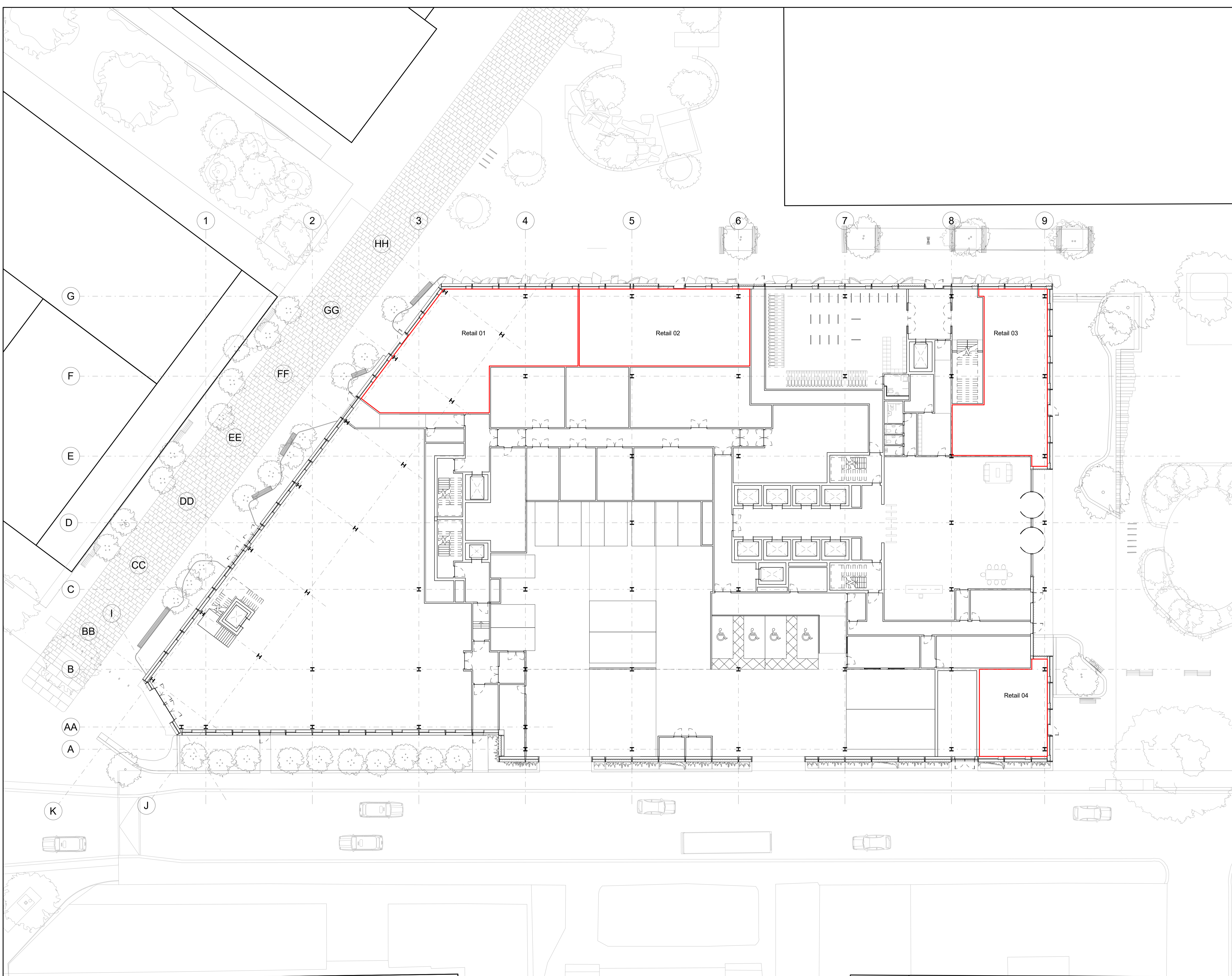
GROUND FLOOR PLAN 1:200 scale
